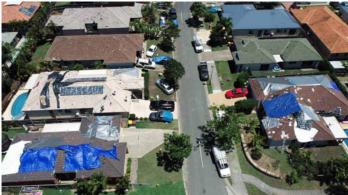
Figure 68: Damage to houses in Springfield, Queensland following a hailstorm on 31 October 2020, where hail in excess of 100mm in diameter was recorded. The damage caused to tile roofs was far greater than the damage to metal roofs, which experienced negligible damage in comparison. Source: QFES.
