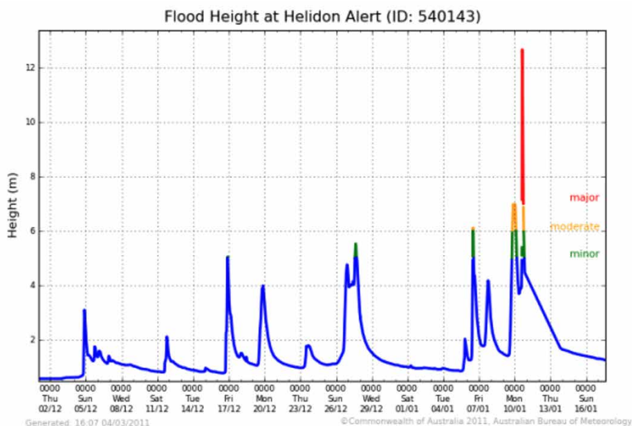
Figure 60. Flood gauge recordings for Helidon. Source: Bureau of Meteorology 107
