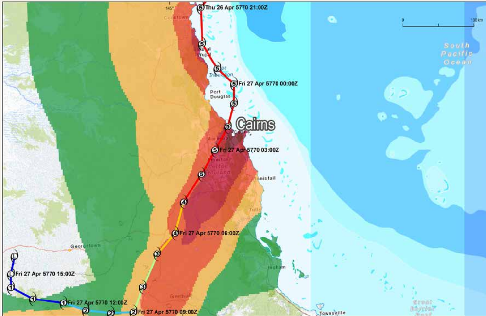
Figure 40: Regional wind field for scenario 013-03564, a Category 5 cyclone impacting Cairns, Qld.
