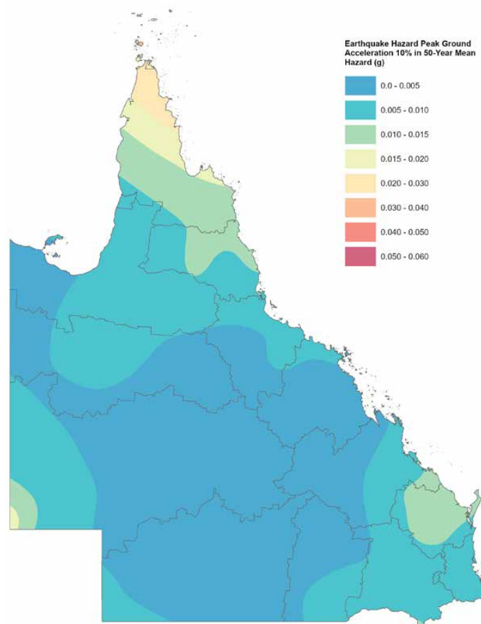
Figure 85: Peak ground acceleration (PGA) of an earthquake with a 10% probability of exceedance within a 50 year period. Source: Geoscience Australia, 2018 330
