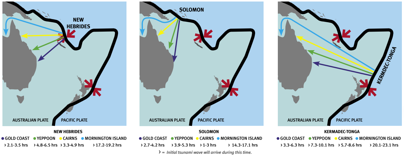
Figure 89: Travel times for regional earthquake-tsunami from the Solomon, New Hebrides and Kermadec-Tonga trenches. Note: These travel times are derived from models and are based on the initial tsunami arrival offshore. They do not consider the time required for the tsunami to propagate close to shore, or the fact that the tsunami may consist of multiple waves lasting for hours or days. Therefore, these travel times are not suitable for determining when the largest waves will arrive, or when the tsunami risk has passed. In the event of an actual tsunami, the Joint Australian Tsunami Warning Centre will include travel times in their warning products. These should be considered the definitive source in the event of a tsunami. Source: produced by QFES with assistance from Geoscience Australia
