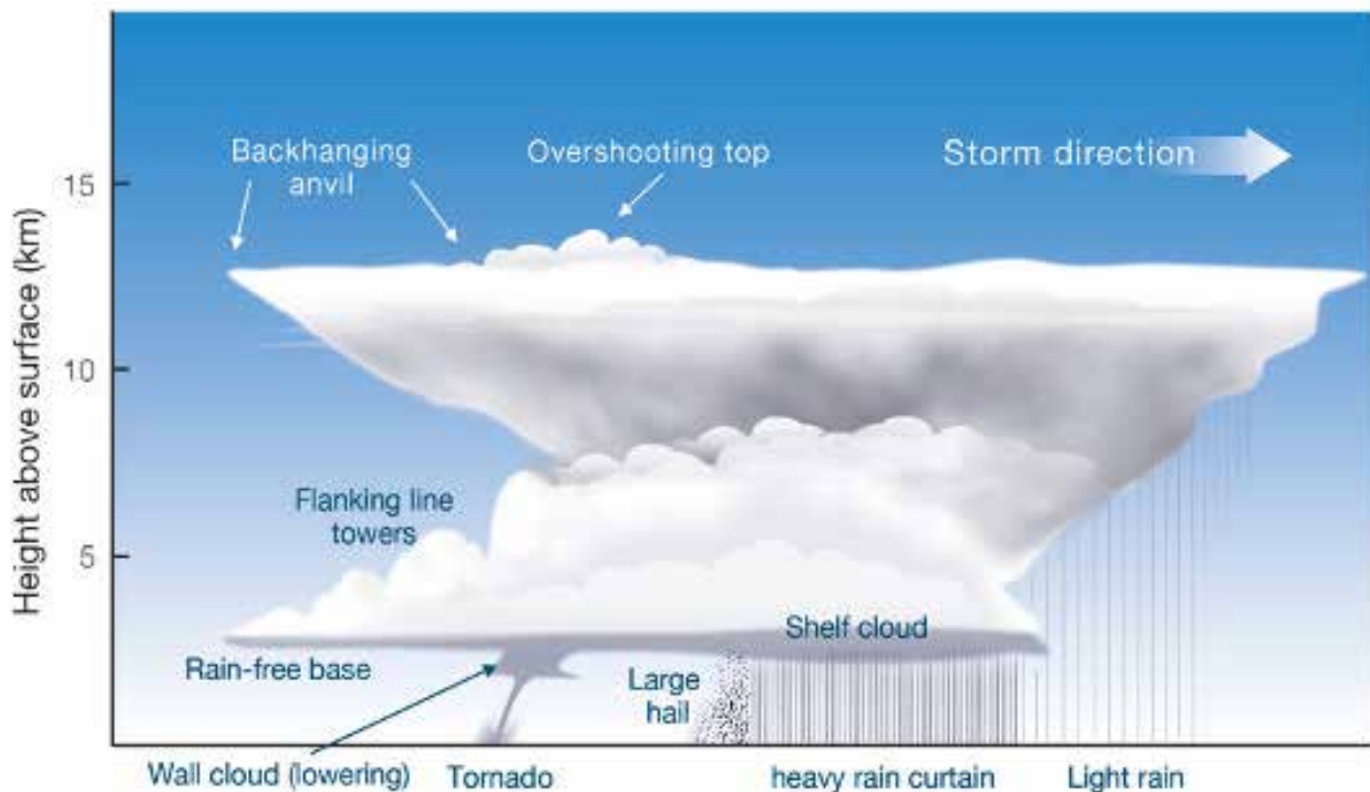
Figure 66: Diagram illustrating some features that may be produced by a severe thunderstorm. Source: the Bureau.
