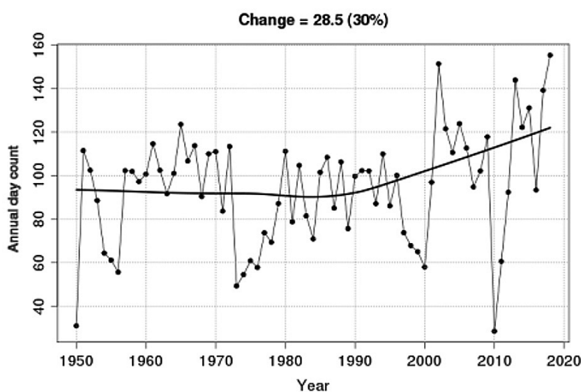
Figure 75: Number of days with an FFDI above 25 for Queensland, from 1950 – 2018. Source: QFES
