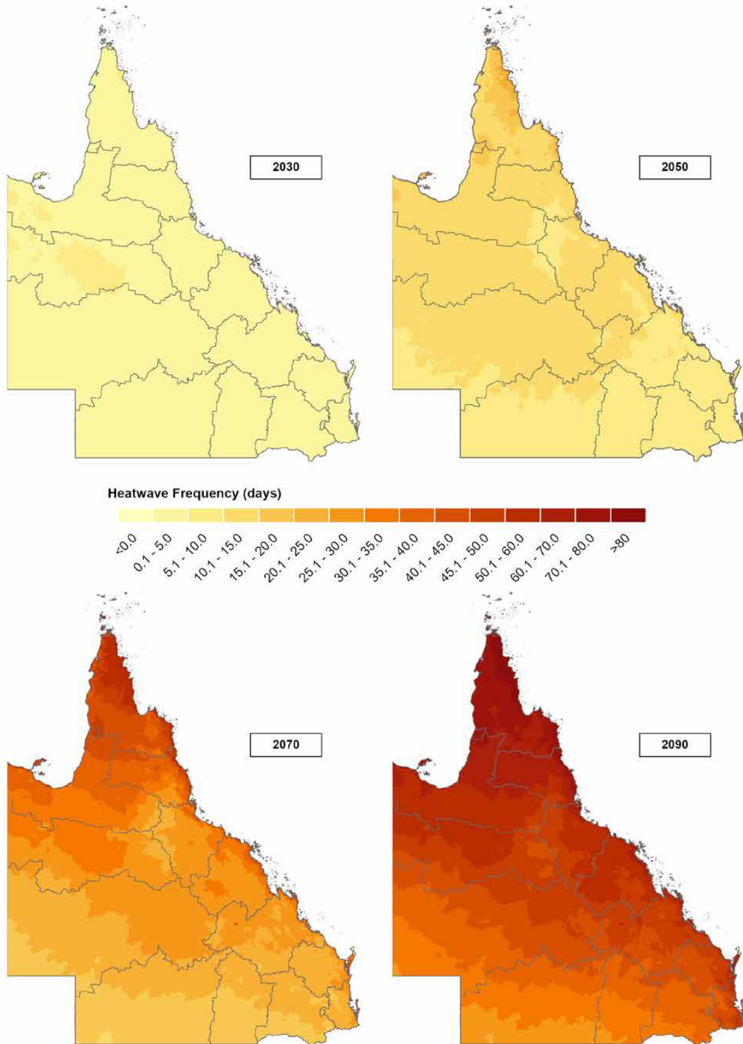
Figures 70: Projections of heatwave frequency (number of days above 1986-2005 baseline) under RCP8.5 for 2030, 2050, 2070, and 2090.
