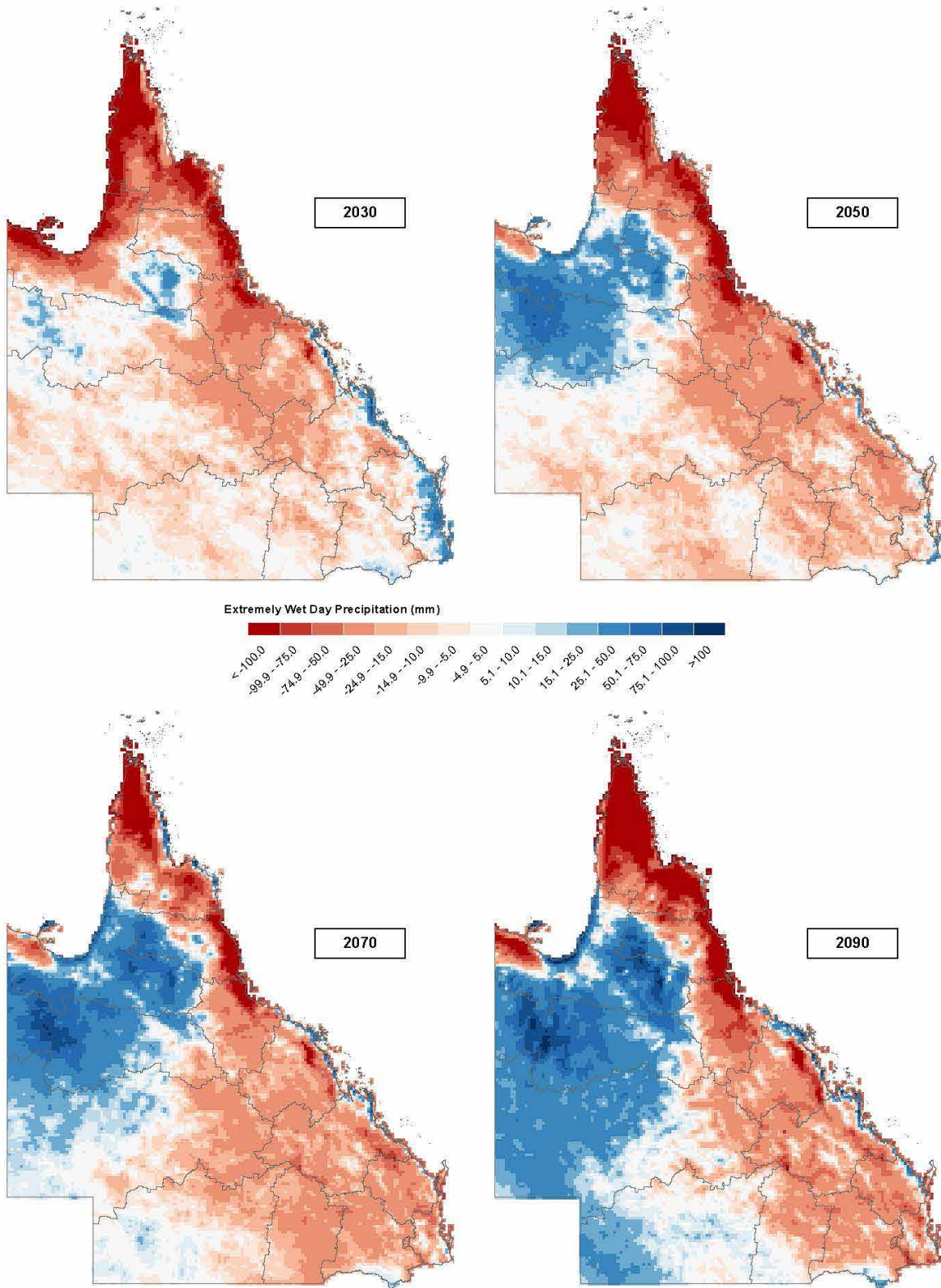
Figures 61: Extremely Wet Day Precipitation for 2030, 2050, 2070, and 2090 using RCP 8.5 (mm change from 1986-2005 baseline). Source: Future Climate Dashboard, Department of Environment and Science.
