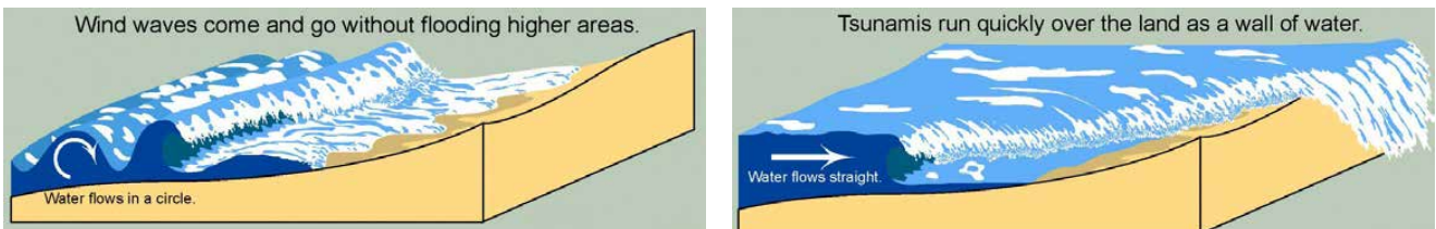
Figure 87: Differences between wind waves and tsunami at the coast. Source: AIDR Tsunami Emergency Planning in Australia Handbook
