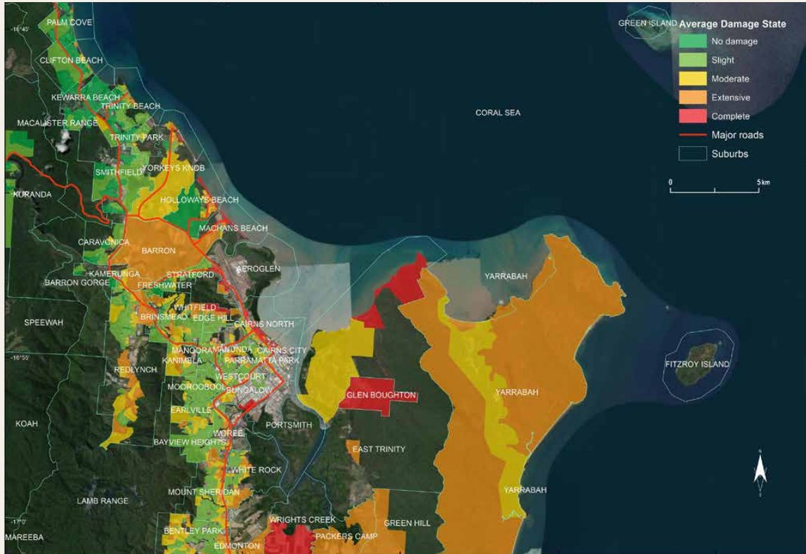
Figure 41: Aggregated residential building damage states for mesh block areas, for scenario 013-03564, a Category 5 cyclone impacting in Cairns, Qld.
