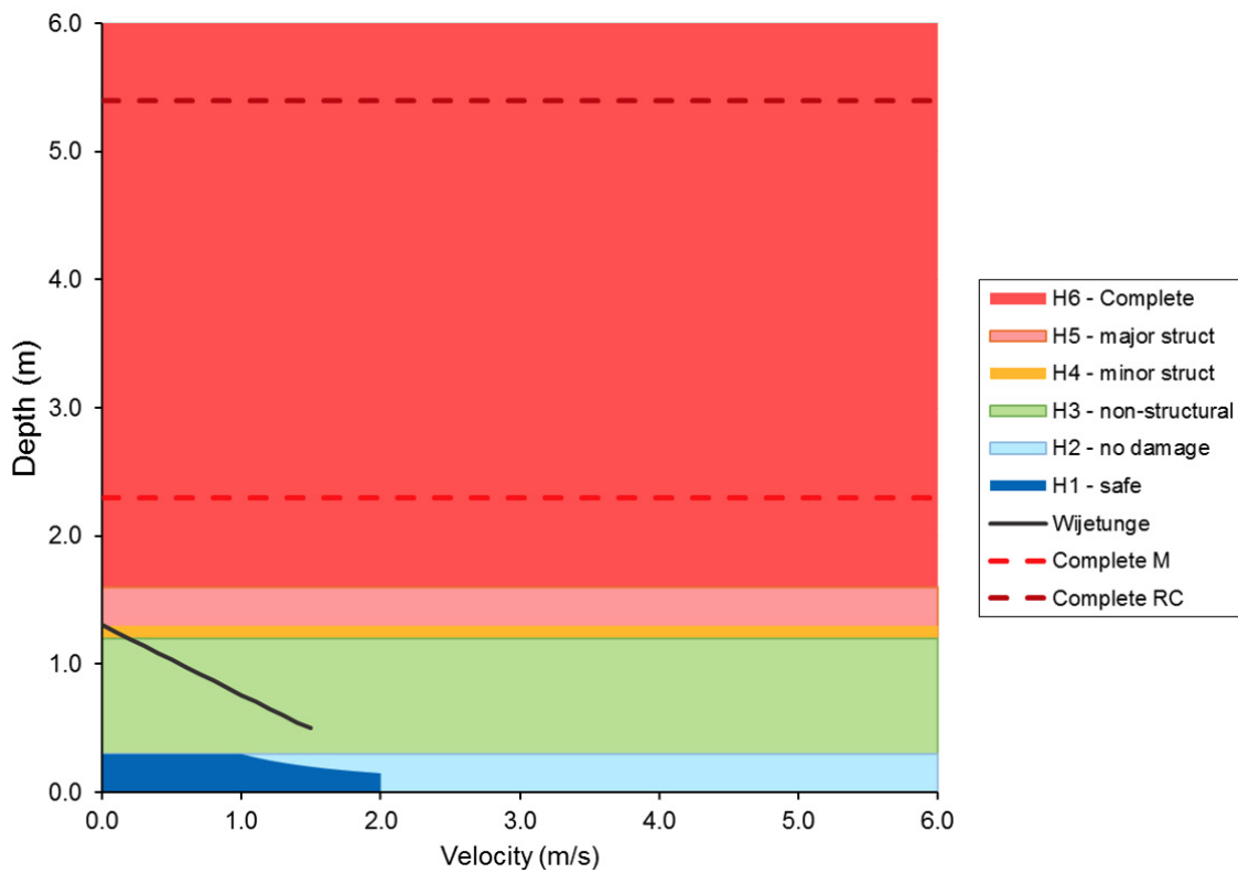
Figure 90: Tsunami hazard curves. Source: DES.
