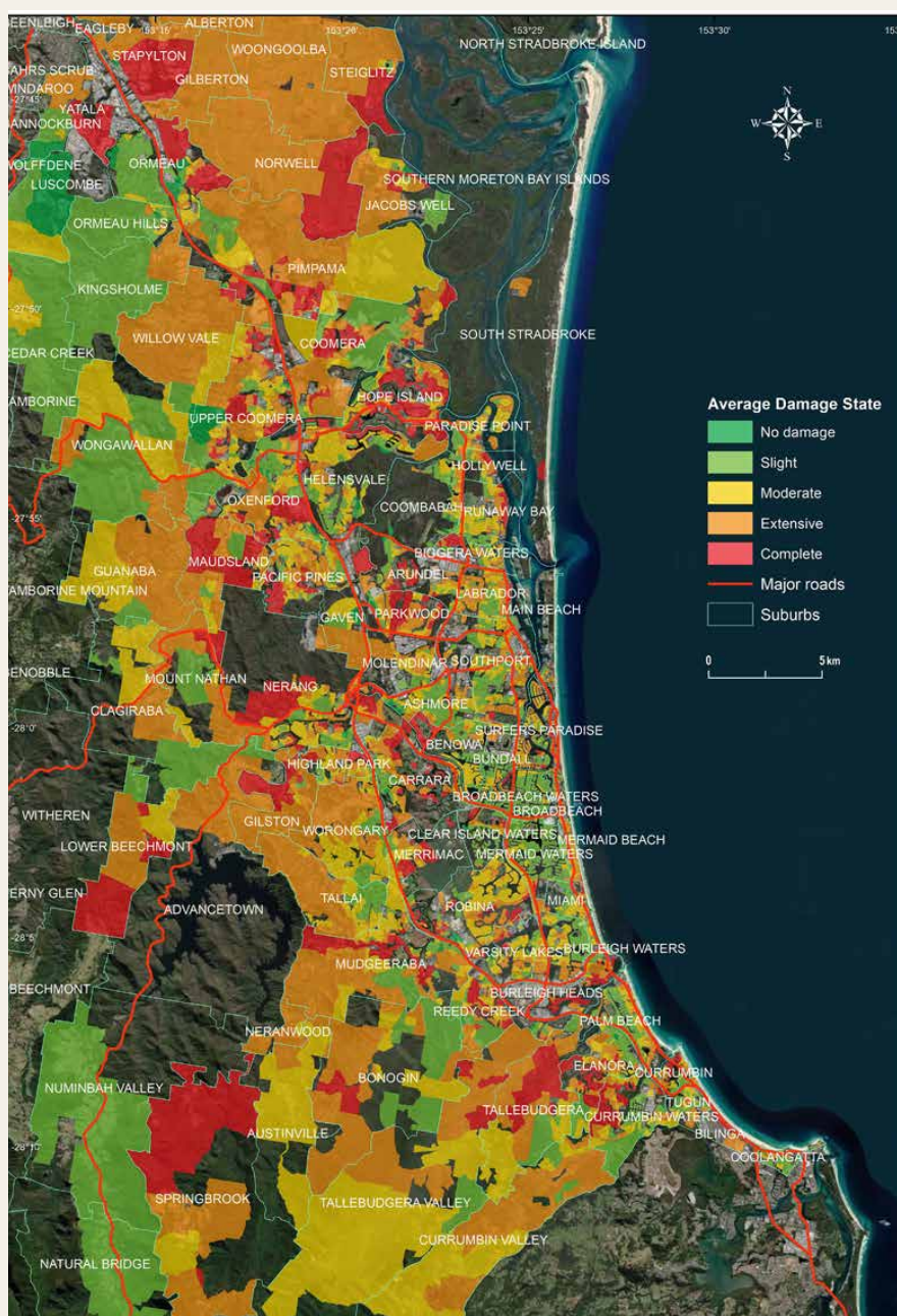
Figure 44: Aggregated residential building damage states for mesh block areas, for scenario 001-00406, a Category 3 cyclone impacting Gold Coast, Qld.
