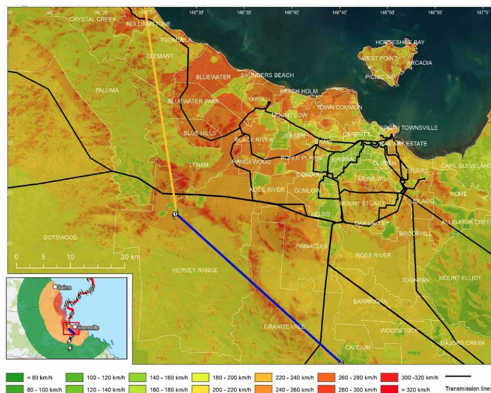
Figure 48: Overview of the transmission and sub-transmission network superimposed over a local wind field for a Category 5 scenario impacting Townsville. Note the position of the network in areas where there is significant acceleration of the cyclonic winds over areas of steep terrain or complex topography.
