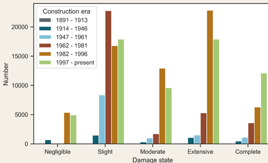
Figure 45: Count of buildings in each damage state, grouped by construction era, for scenario 001-00406, a Category 3 cyclone impacting Gold Coast, Qld.
