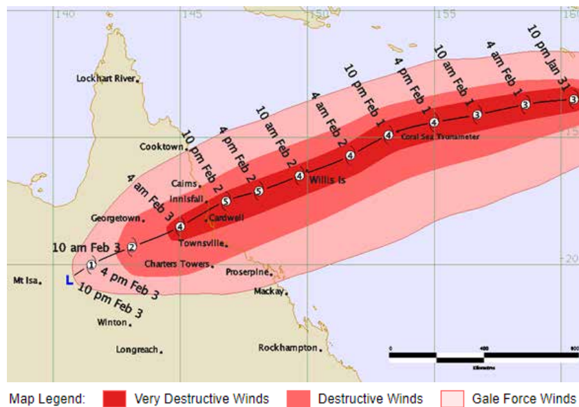
Figure 19: Track and Intensity Information for Tropical Cyclone Yasi. Source: reproduced with permission from the Bureau of Meteorology.
