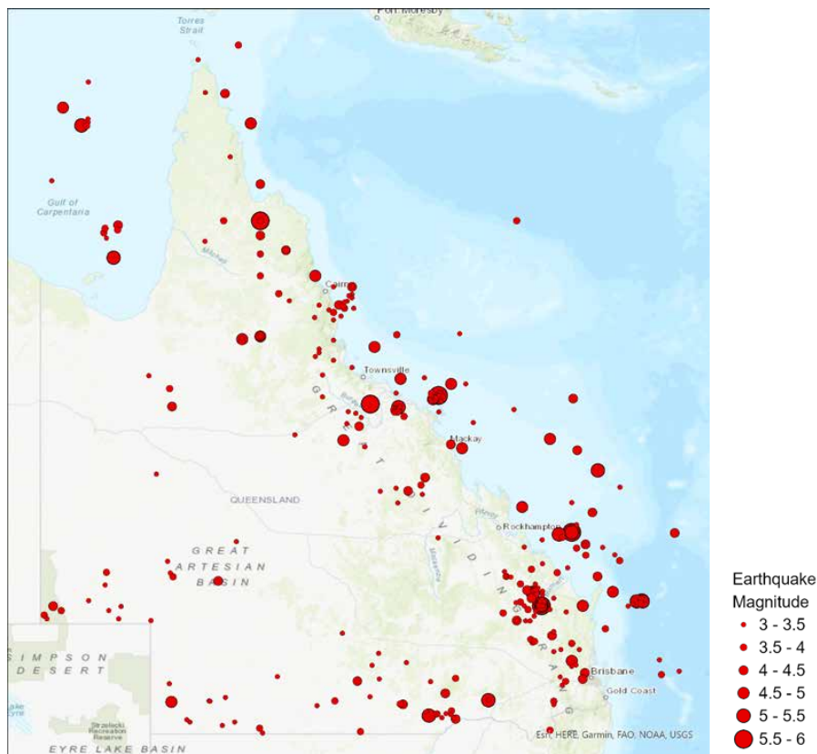
Figure 83: Locations of recorded earthquakes in Queensland, between 1866 and 2020. The size of the points represents the magnitude of the earthquake. Source: Data from Geoscience Australia.
