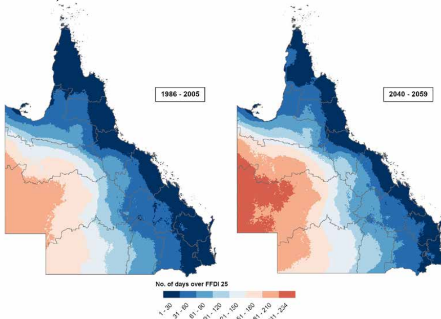
Figure 78: FFDI projections showing number of days above FFDI 25 for a historical time period (1986-2005) and for 2040-2059.
