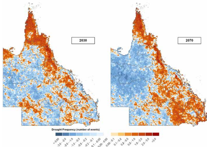
Figure 111: Climate projections for drought frequency under RCP8.5 for 2030 and 2070. Climate data sourced from the Department of Environment and Science.
