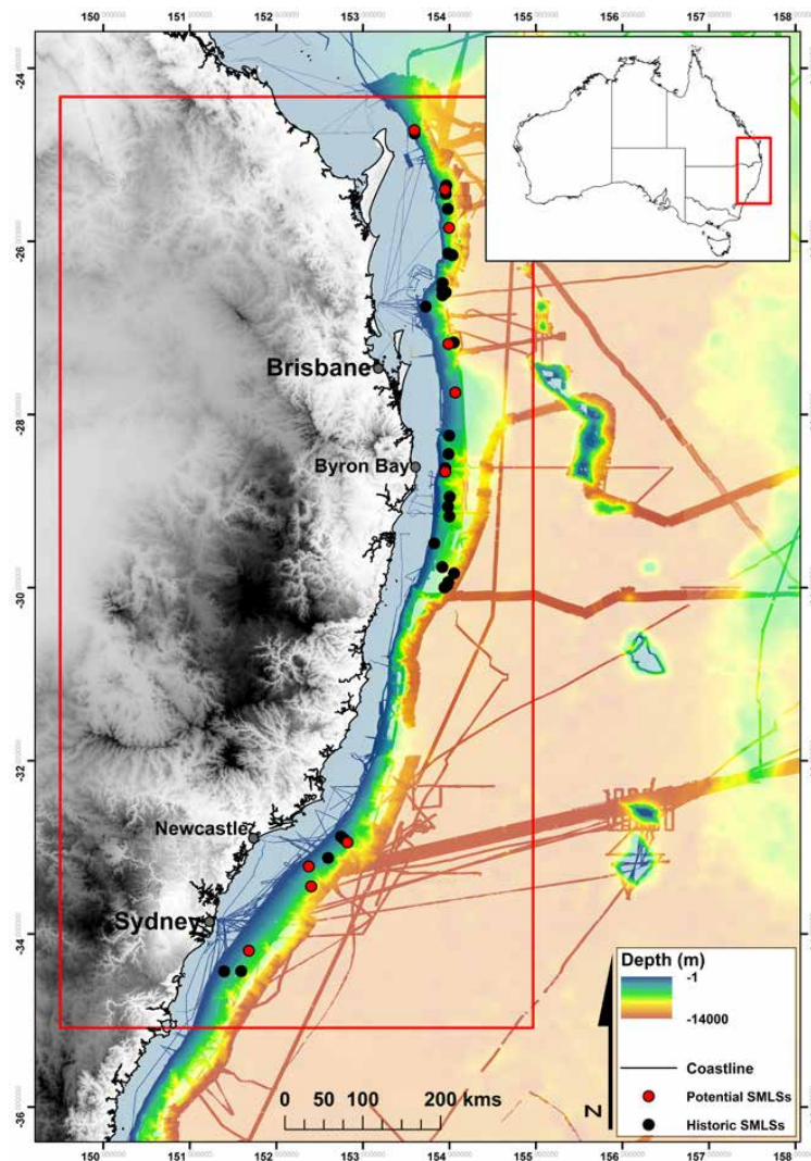
Figure 91: This illustration shows the location of historic submarine landslides with tsunamigenic potential (black dots) and potential future submarine landslides sites (red dots) identified by Clarke (2014) along the east Australian continental margin. The red box outlines the region containing submarine landslides with tsunamigenic potential. Slides with tsunamigenic potential were defined as those with dimensions of 50-250m thick, 1km to >10km wide and in depths of 500-2500m. Source: Clarke et al. (2018)
