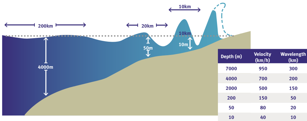
Figure 88: Wave characteristics in the open ocean and near shore. Sourced and adapted from: AIDR Tsunami Emergency Planning in Australia Handbook
