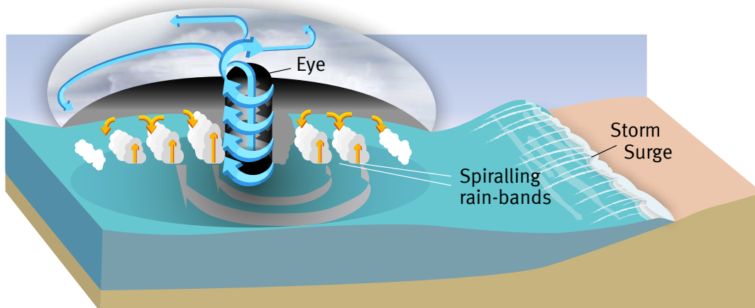
Figure 20: Diagram of a tropical cyclone system.
