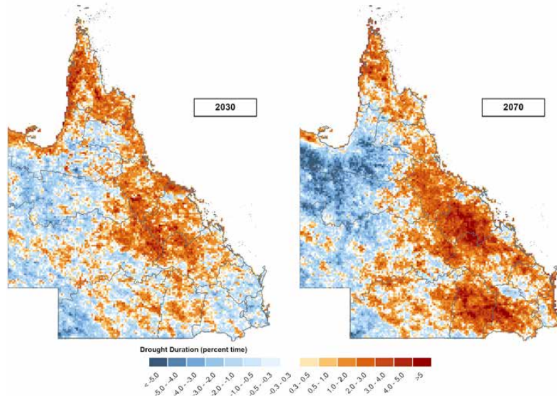
Figure 110: Climate projections for drought duration under RCP8.5 for 2030 and 2070. Climate data sourced from the Department of Environment and Science.
