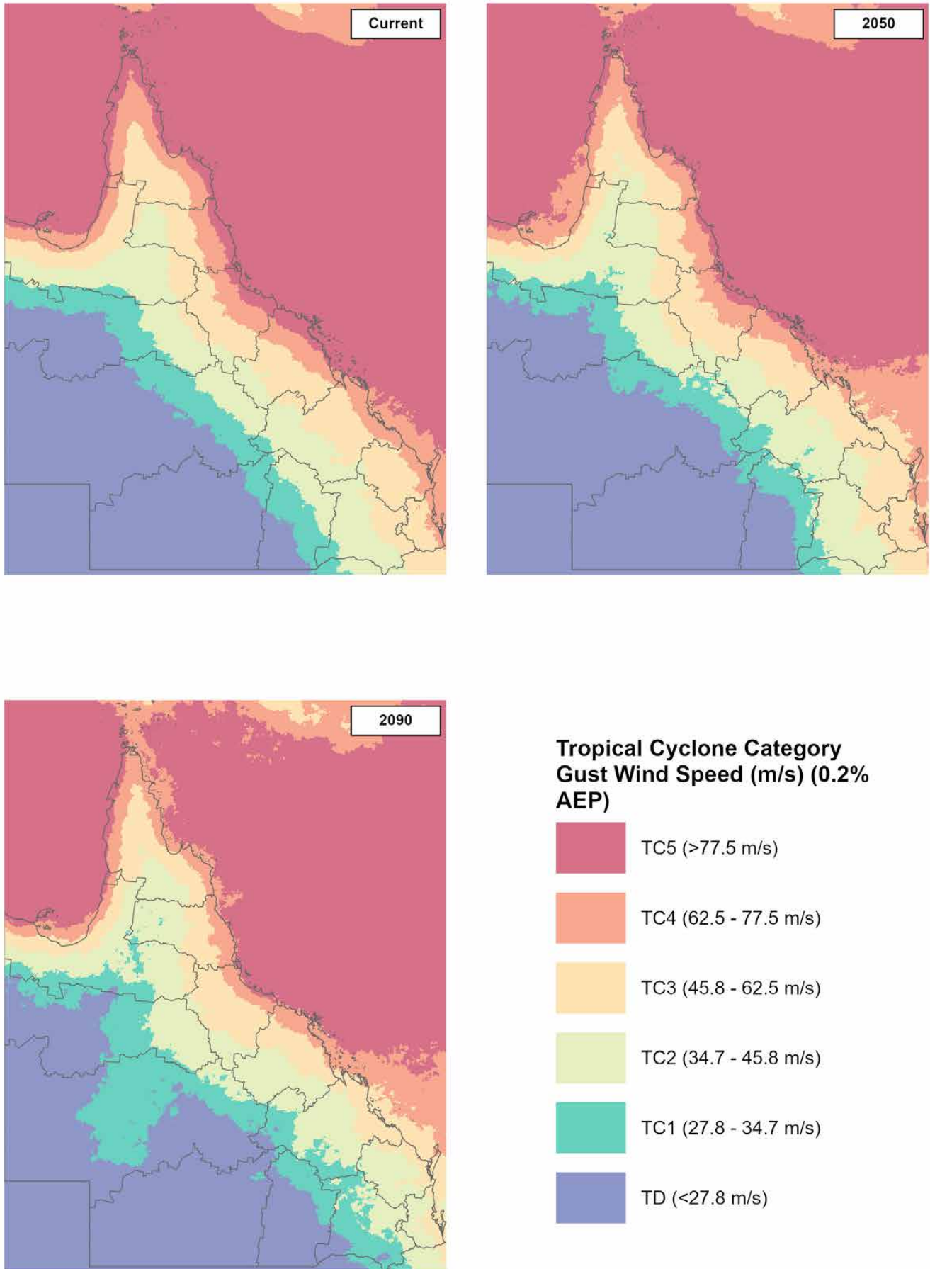
Figure 37: Projections of tropical cyclone intensity of an AEP 0.2% event using RCP8.5 for current, 2050 and 2090 time periods.
