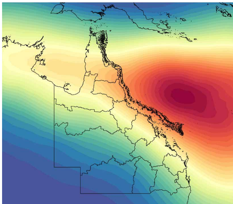
Figure 23: Density of tropical cyclone tracks between 1921 and 2021, with outlines of regional planning areas and the Great Barrier Reef. Data from IBTRACS. 64 Red indicates greater cyclone activity, and blue indicates lesser. Source: QFES.
