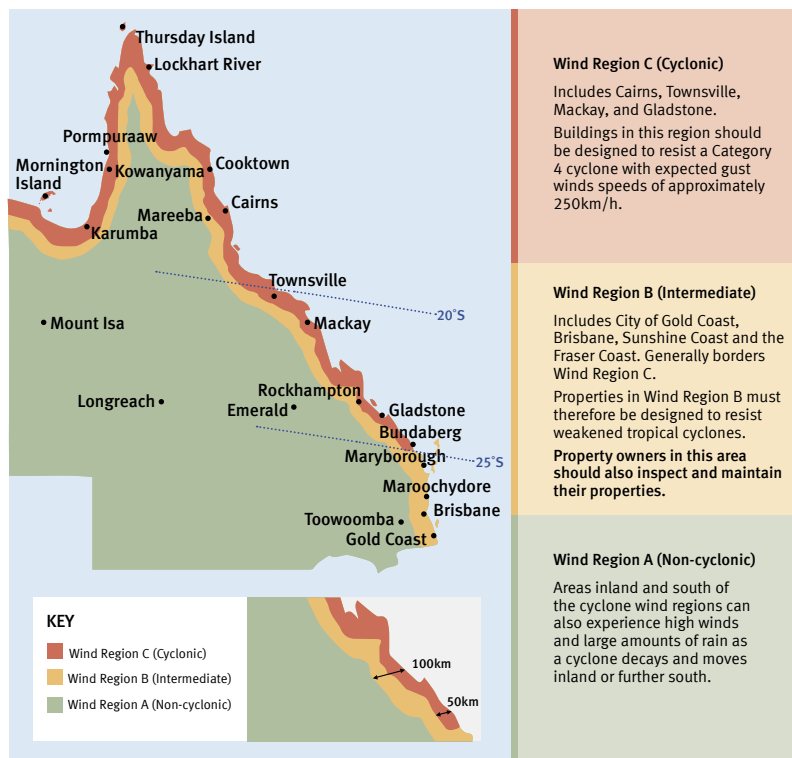
Figure 18: AS/NZS 1170.2 2011 Wind Regions for Queensland, with key locations marked (after AS/NZS 1170.2, 2011).
